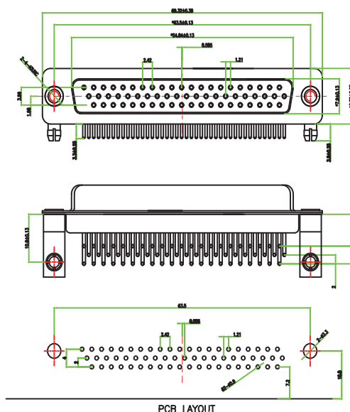
PCB LAYOUT
