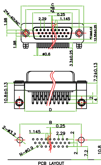
PCB LAYOUT
